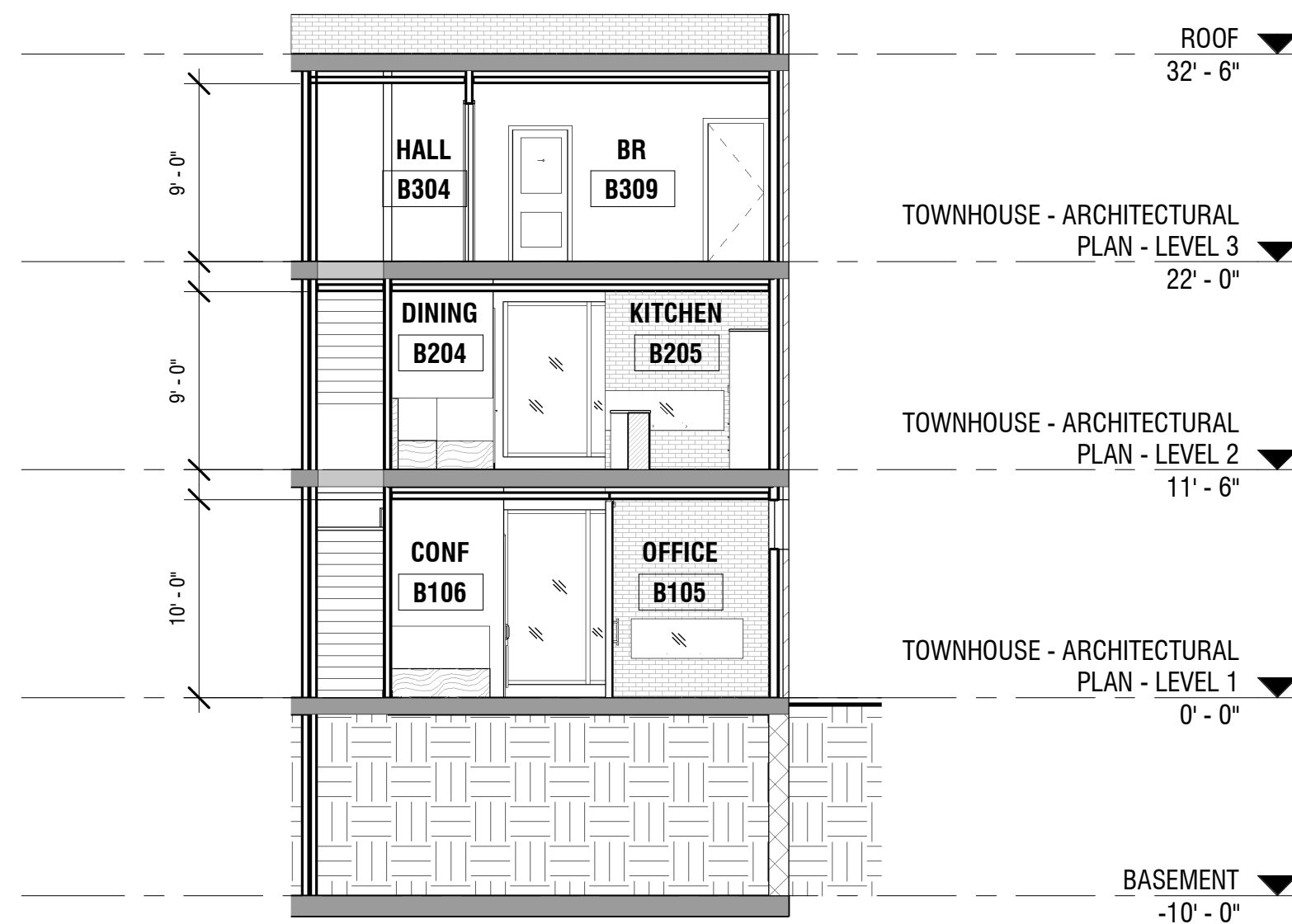
② TOWNHOUSE - TRANSVERSE SECTION 1/8" = 1'-0"
