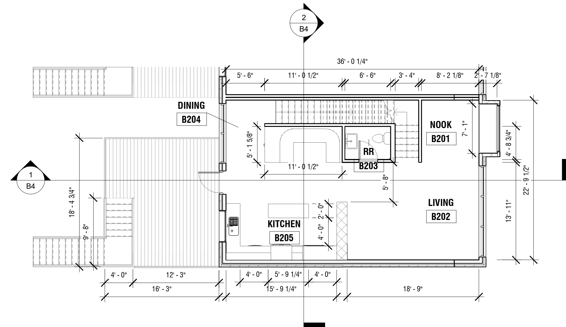
② TOWNHOUSE - ARCHITECTURAL PLAN - LEVEL 2 1/8" = 1'-0"
