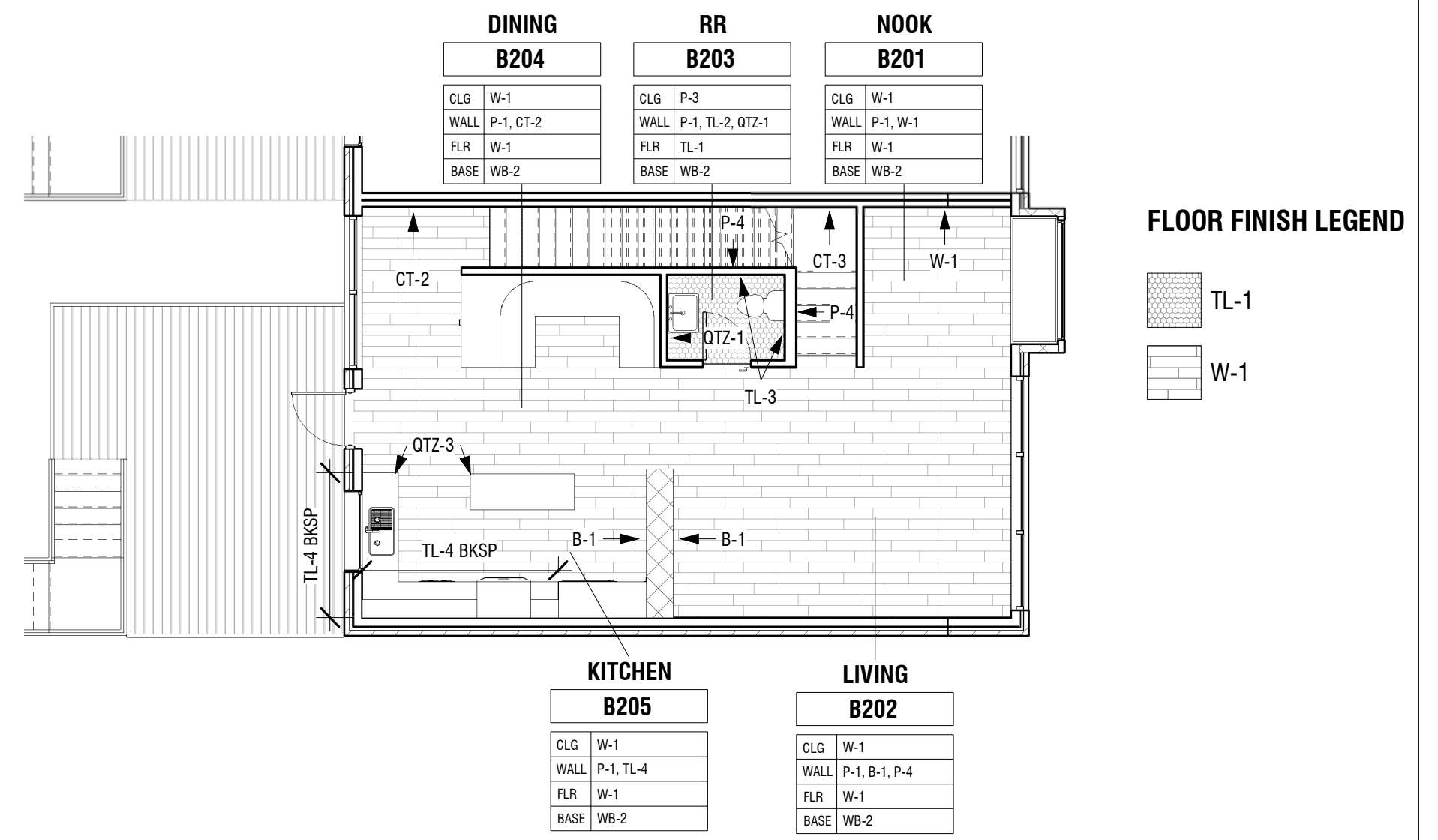
3 TOWNHOUSE - FINISH PLAN - LEVEL 2 1/8" = 1'-0"
