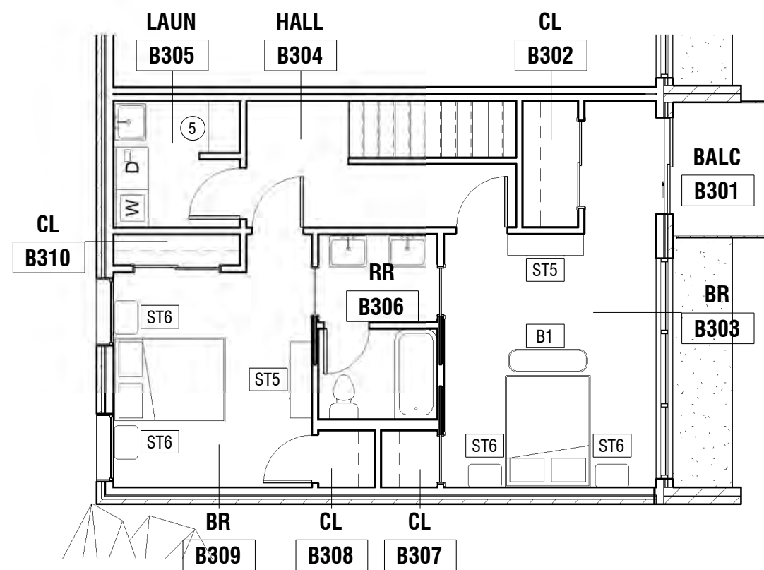
3 TOWNHOUSE - FURNITURE PLAN - LEVEL 3 1/8" = 1'-0"
