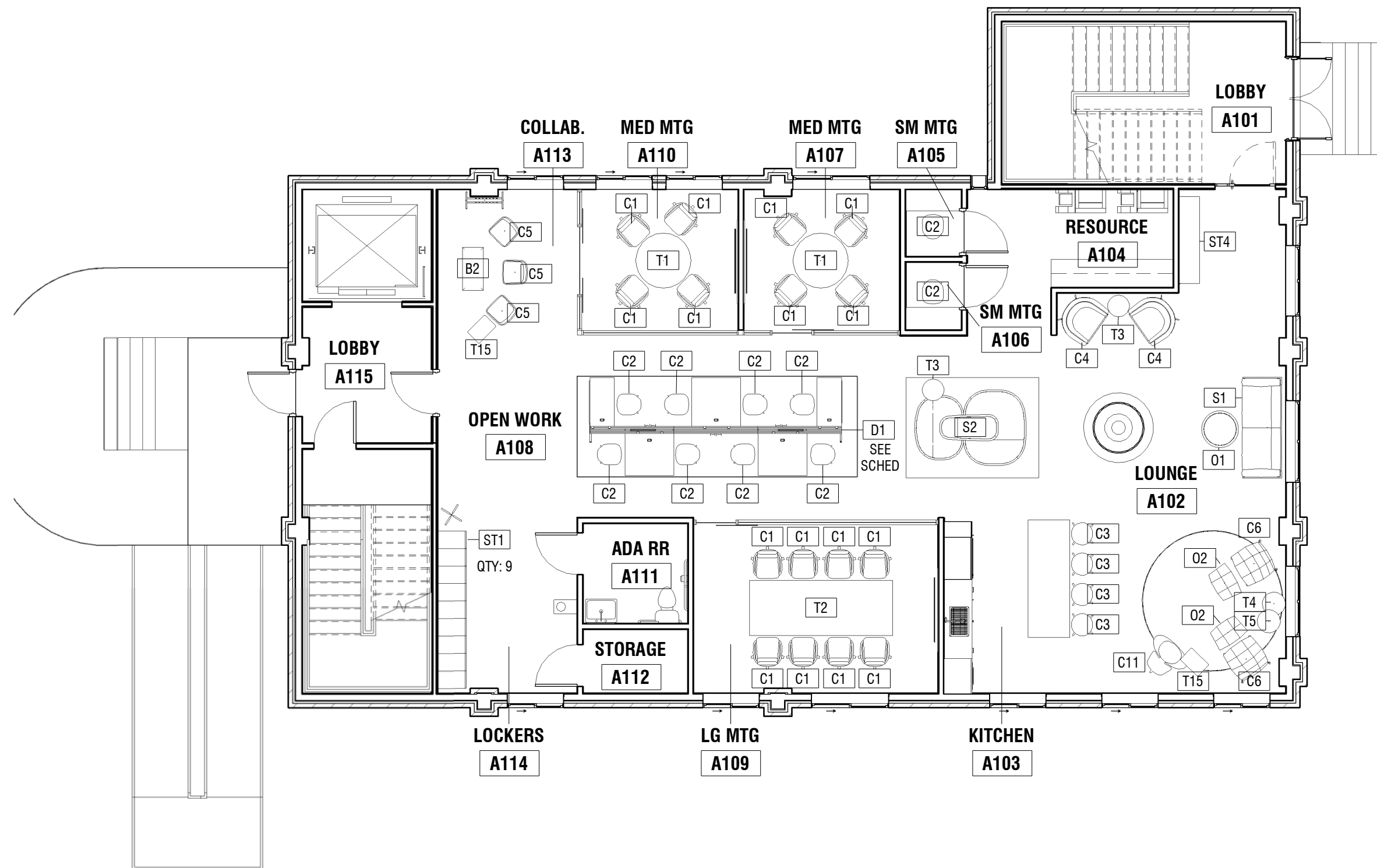
① COWORKING - FURNITURE PLAN 1/8" = 1'-0"
