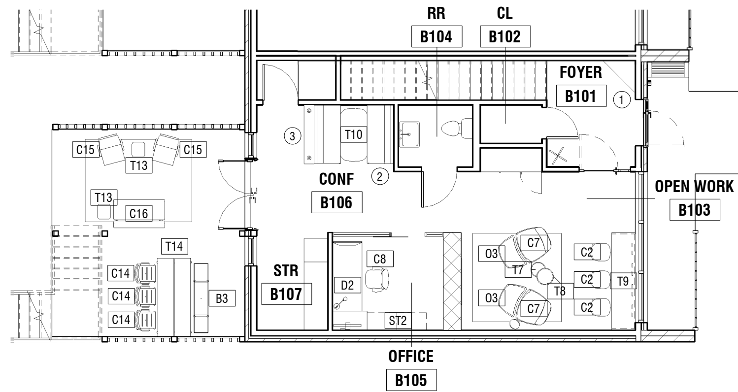
1 TOWNHOUSE - FURNITURE PLAN - LEVEL 1 1/8" = 1'-0"
