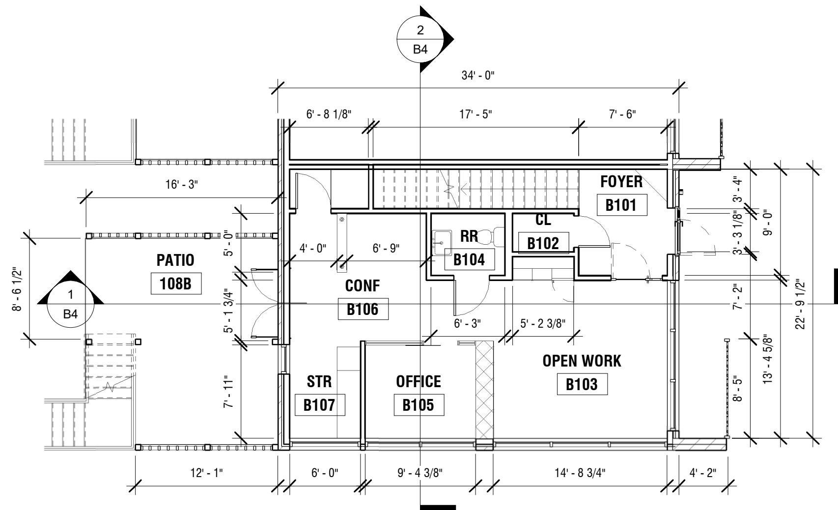
① TOWNHOUSE - ARCHITECTURAL PLAN - LEVEL 1 1/8" = 1'-0"
