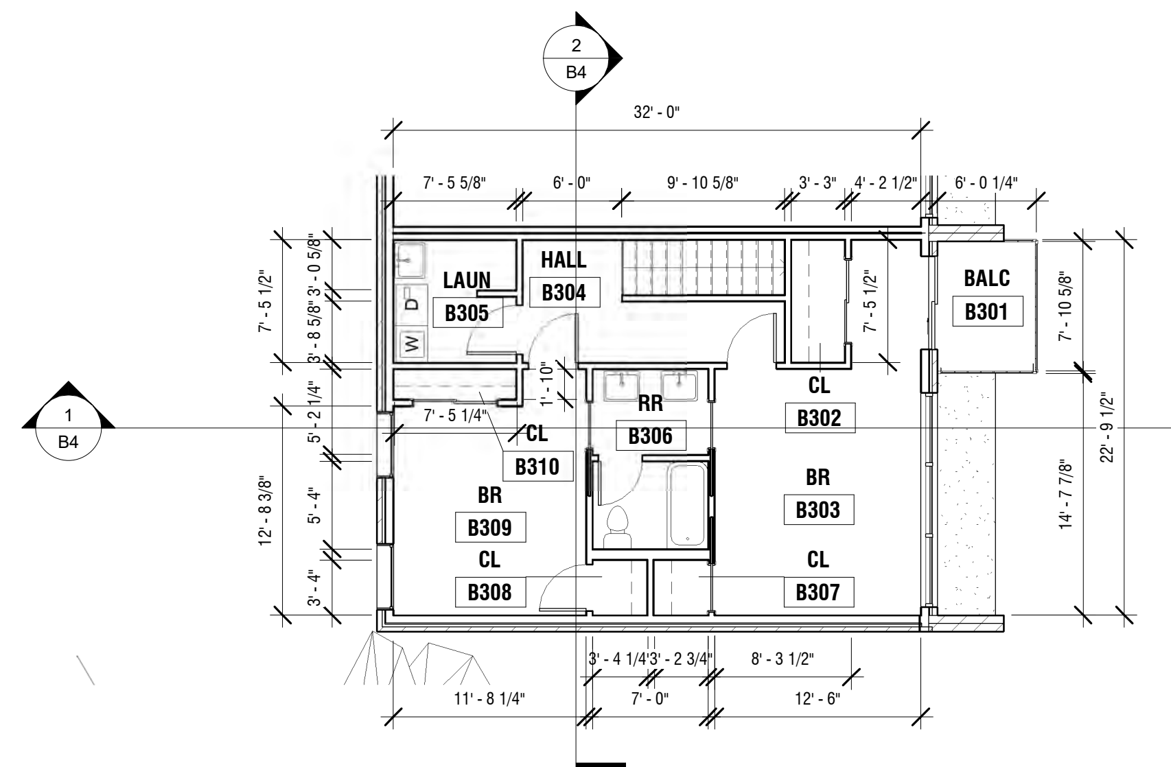
③ TOWNHOUSE - ARCHITECTURAL PLAN - LEVEL 3 1/8" = 1'-0"
