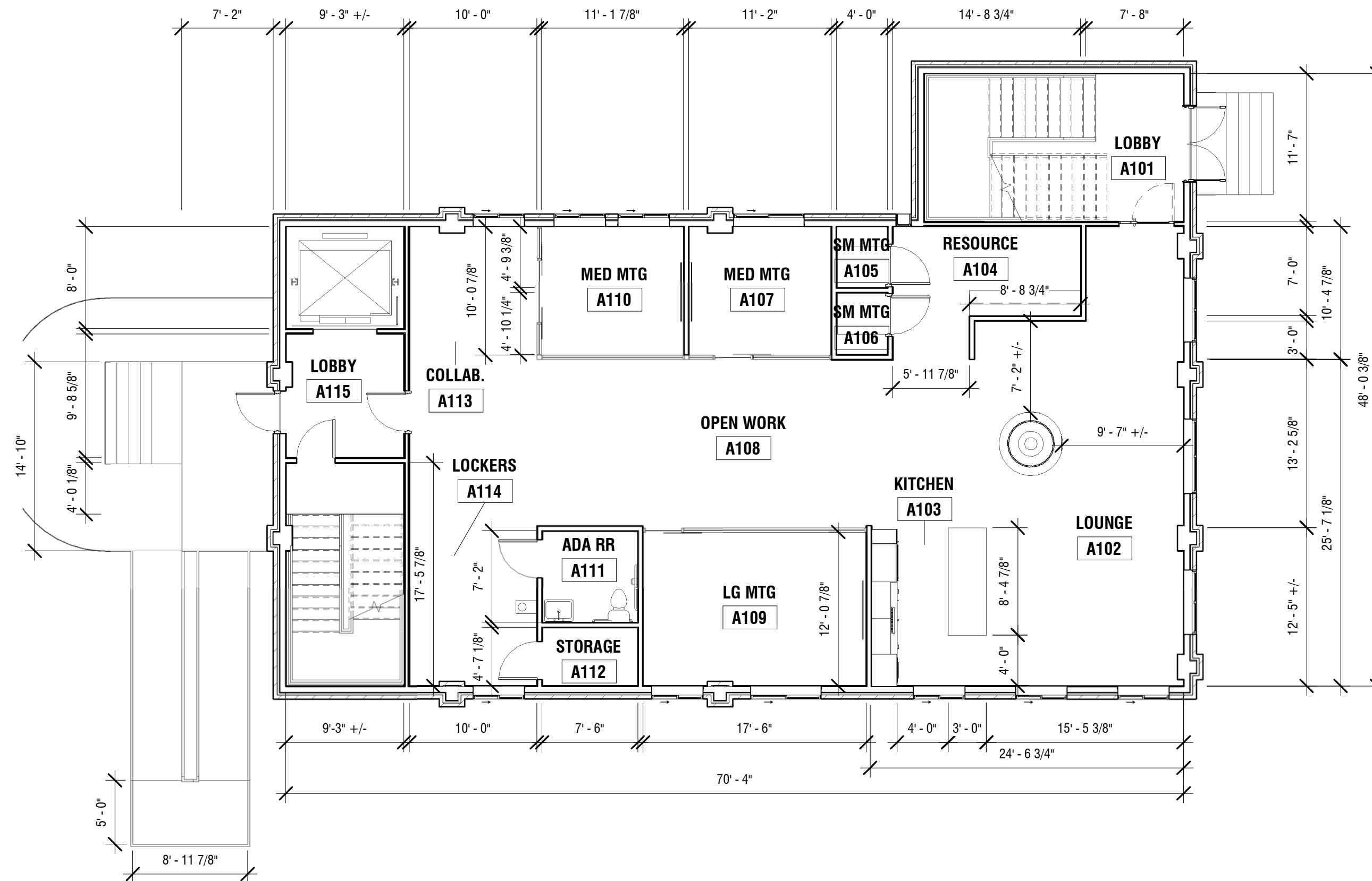
1 COWORKING - ARCHITECTURAL PLAN 1/8" = 1'-0"
