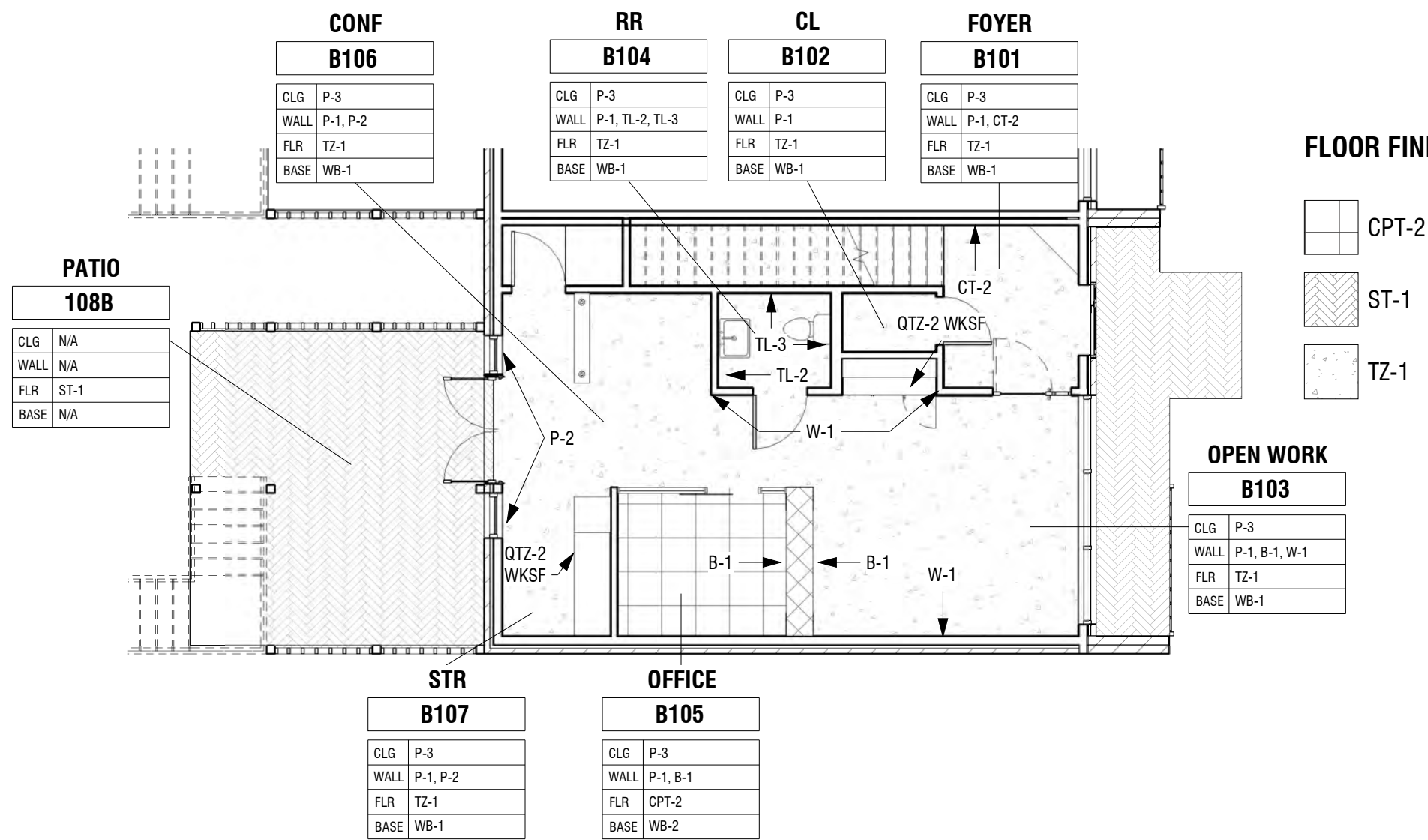
2 TOWNHOUSE - FINISH PLAN - LEVEL 1 1/8" = 1'-0"
