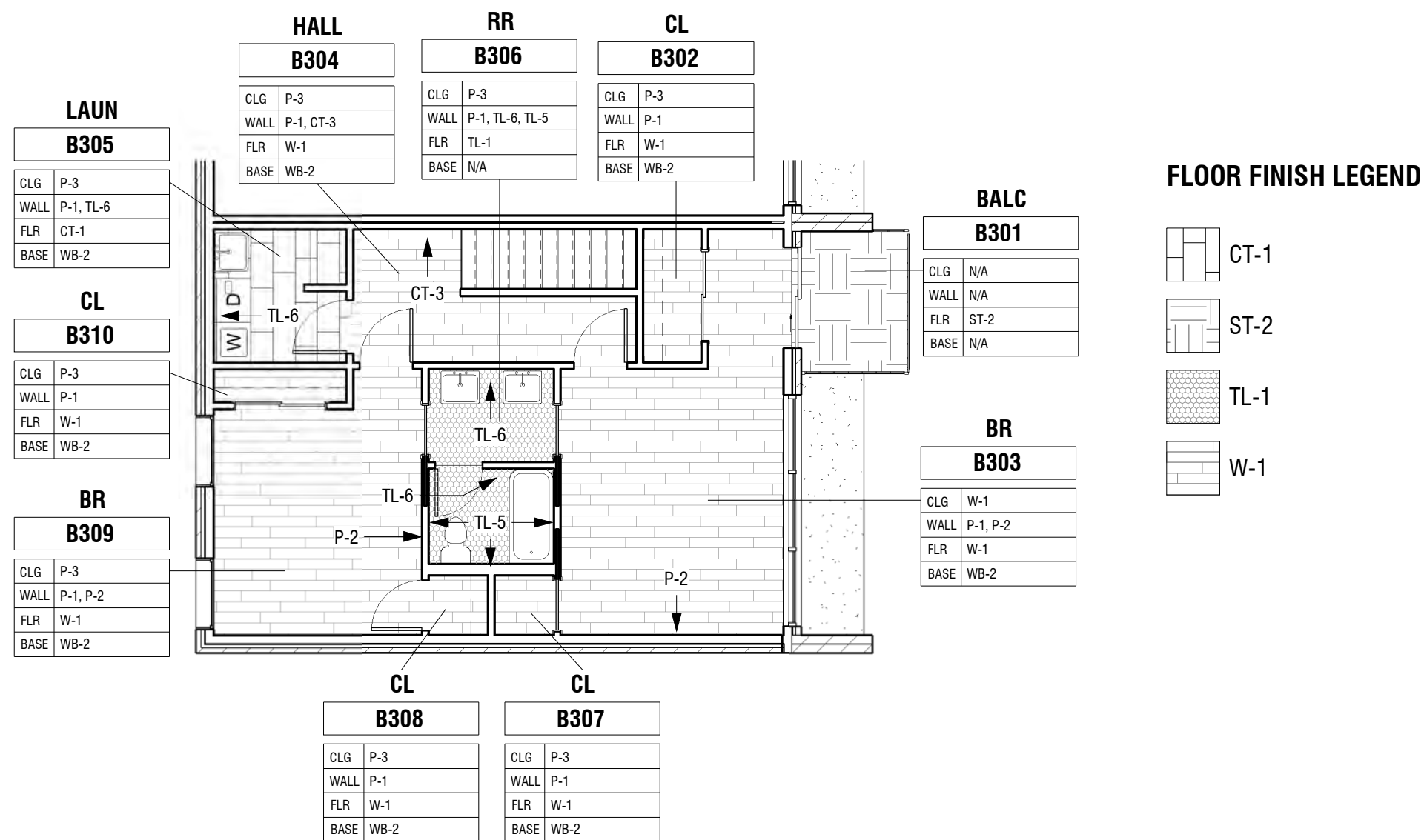
1 TOWNHOUSE - FINISH PLAN - LEVEL 3 1/8" = 1'-0"
