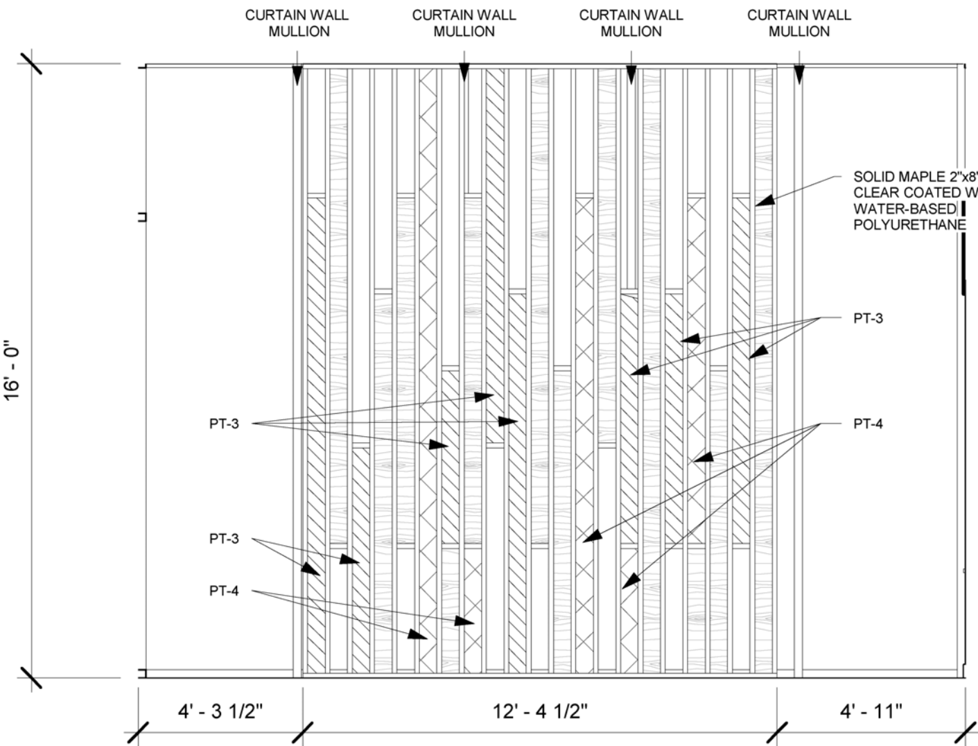
CUSTOM ROOM DIVIDER DETAIL
