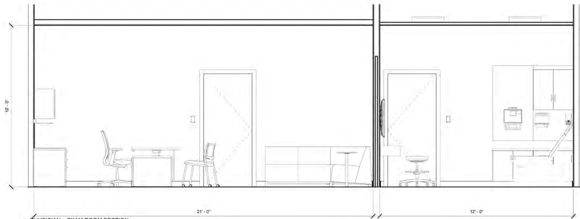
③ PHYSICIAN + EXAM ROOM SECTION 1/2" = 1'-0"
