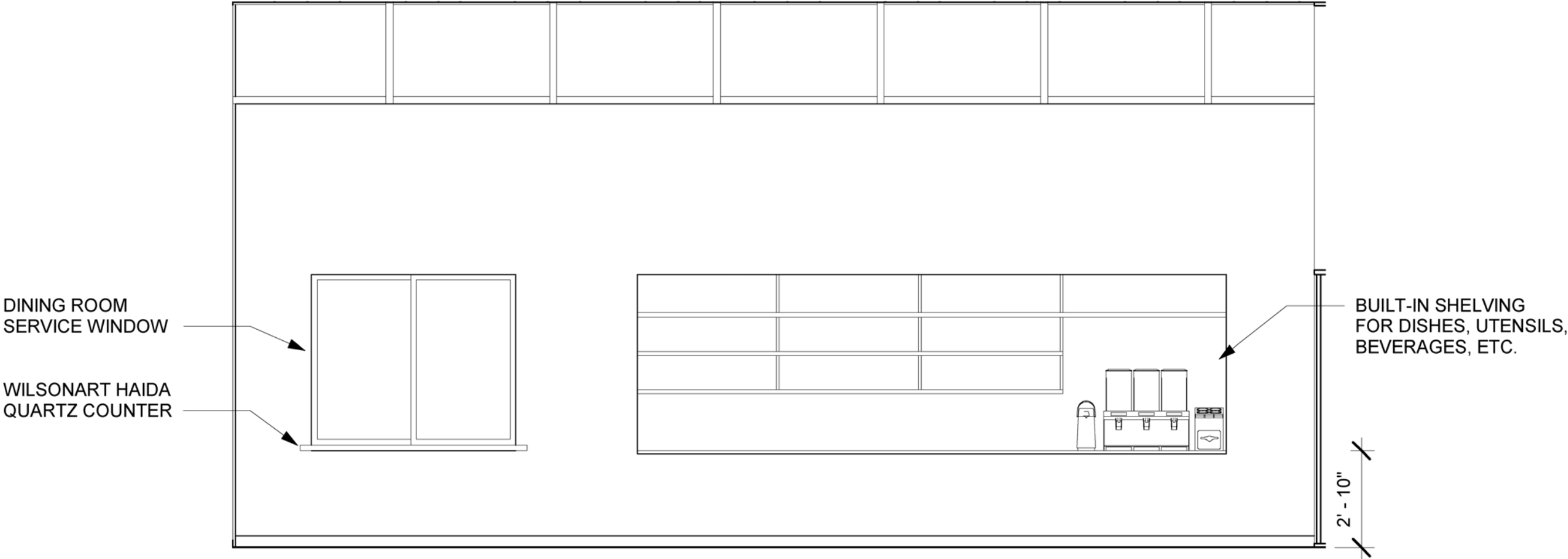
② DINING ROOM ELEVATION 1/4" = 1'-0"
