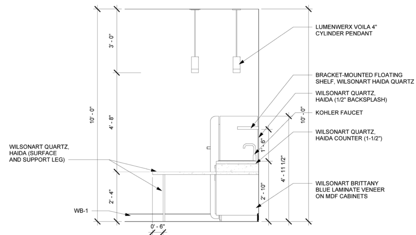
④ APT KITCHEN ELEVATION DETAIL - B 1/2" = 1'-0"
