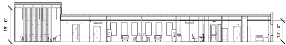
② TRANSVERSE BUILDING SECTION 1/16" = 1'-0"
