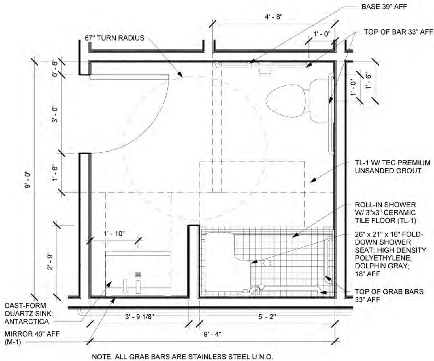
ENLARGED RESIDENT (ACCESSIBLE) BATHROOM FLOORPLAN
