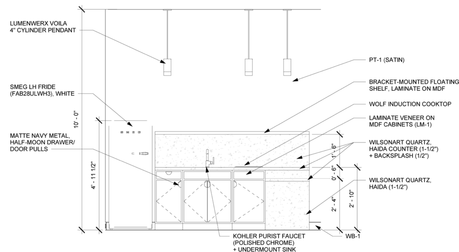
② APT KITCHEN ELEVATION DETAIL - A 1/2" = 1'-0"
